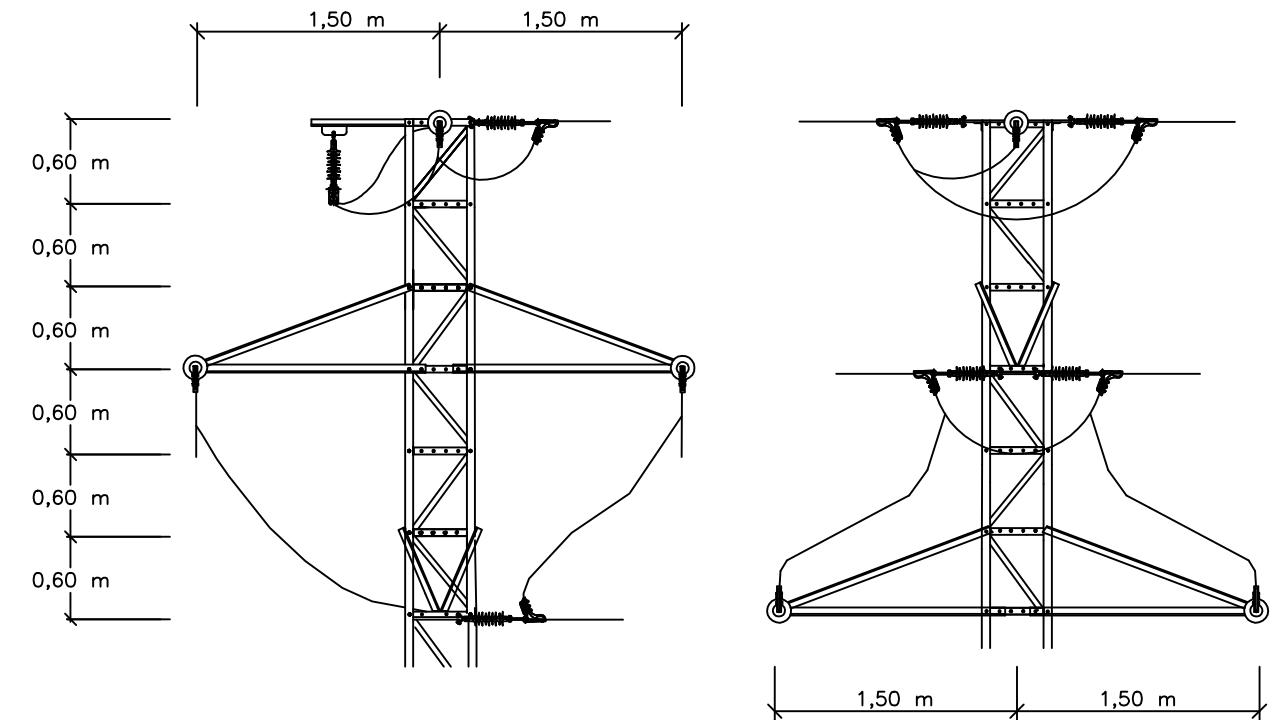
ARMAT TRIANGLE AMARRE TR2 (Pos 3) + TR2 (Pos 6) a nou CT (detall armat del suport S/N)
